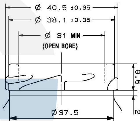
NECK FINISH DETAILS
